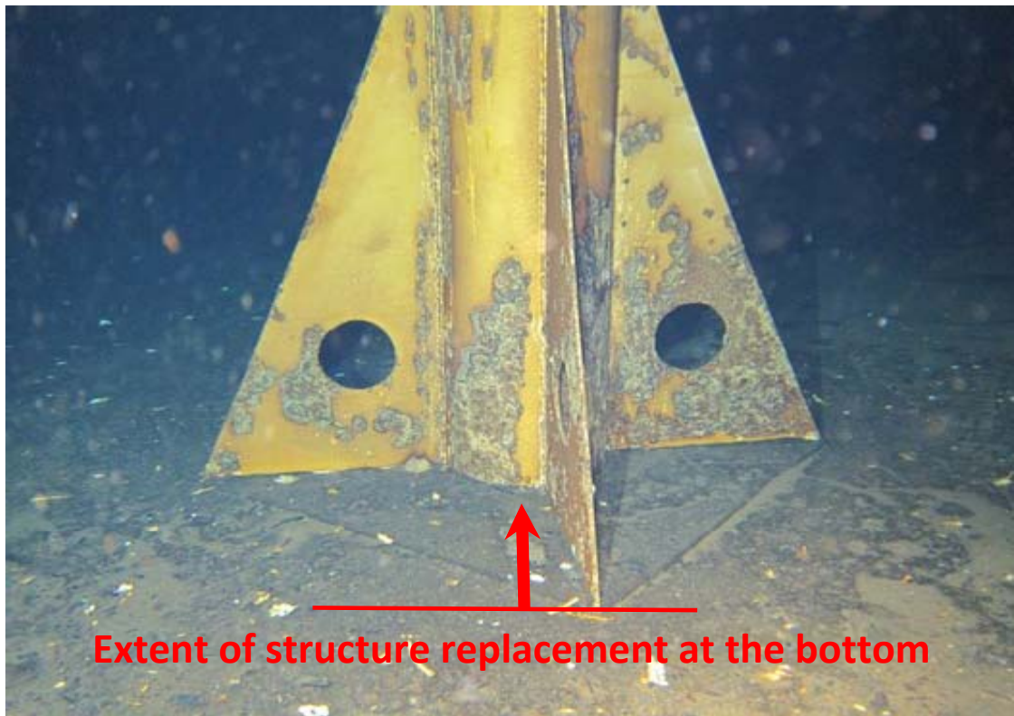
MG#2 center column base plate and extent of roof structure replacement at the bottom.
