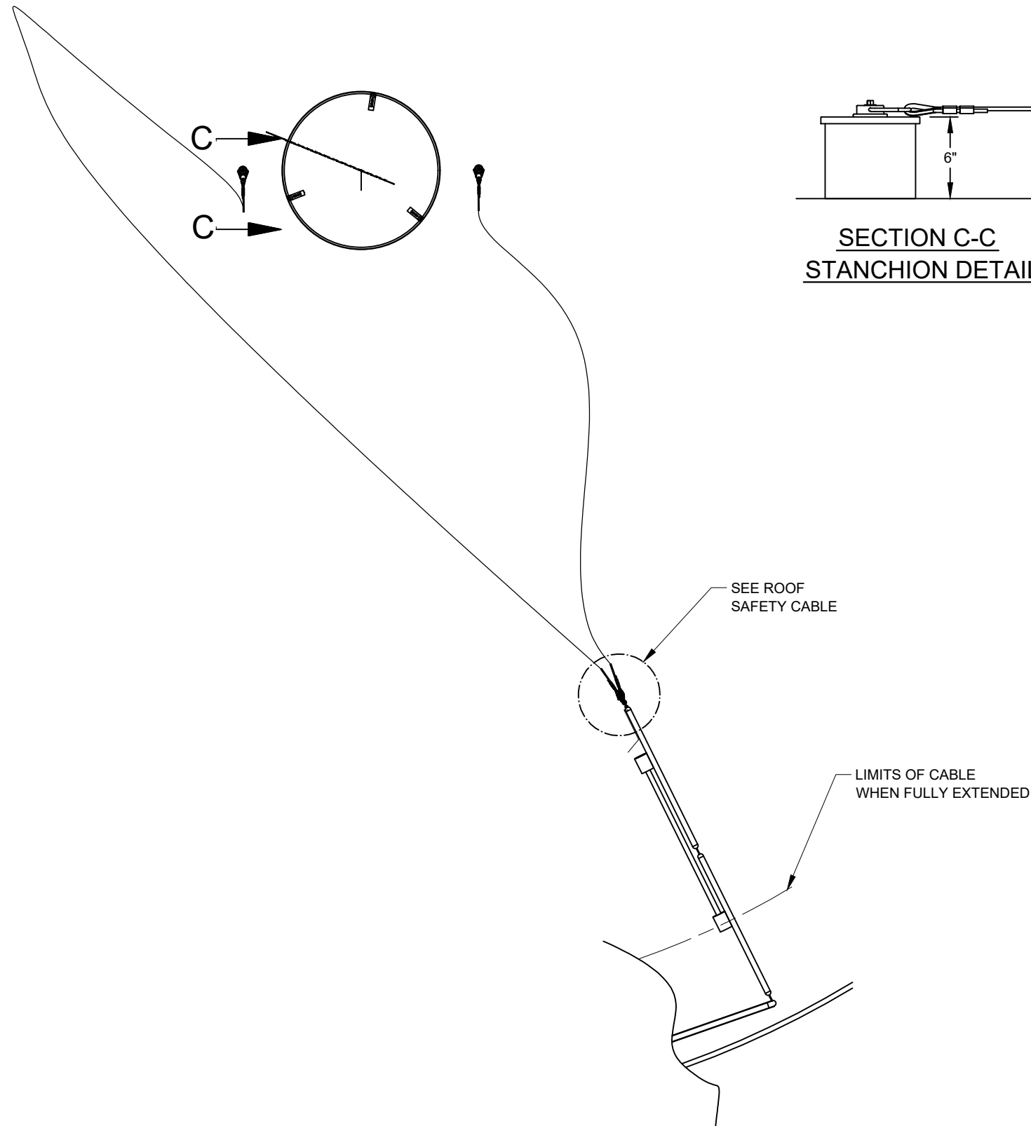
ROOF GUARDRAIL-PLAN
